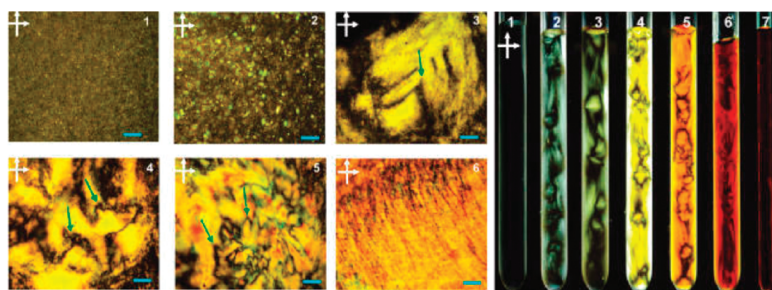
Figure 3. Polarized optical microscopy planar images of various GO suspensions showing distinct Schlieren textures. The arrows point to singularities and biphasic regions. The right panel shows crossed polarizers of GO suspensions of different concentrations in test tubes. Reproduced from ref 5. Copyright 2011 American Chemical Society.
